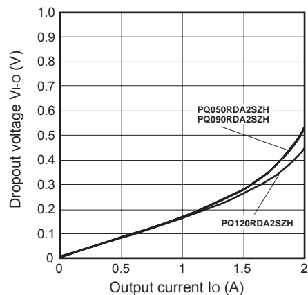
Fig.16 Dropout Voltage V_{I-O} vs. Output Current (PQxxxRDA2SZH)
